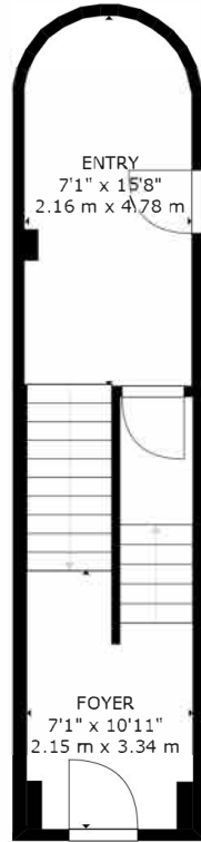
FLOOR 2
